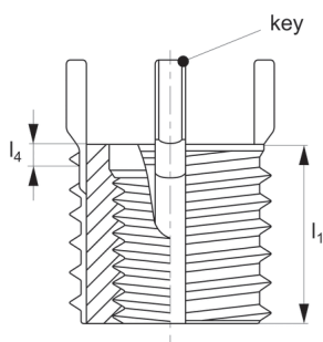
non-locking
